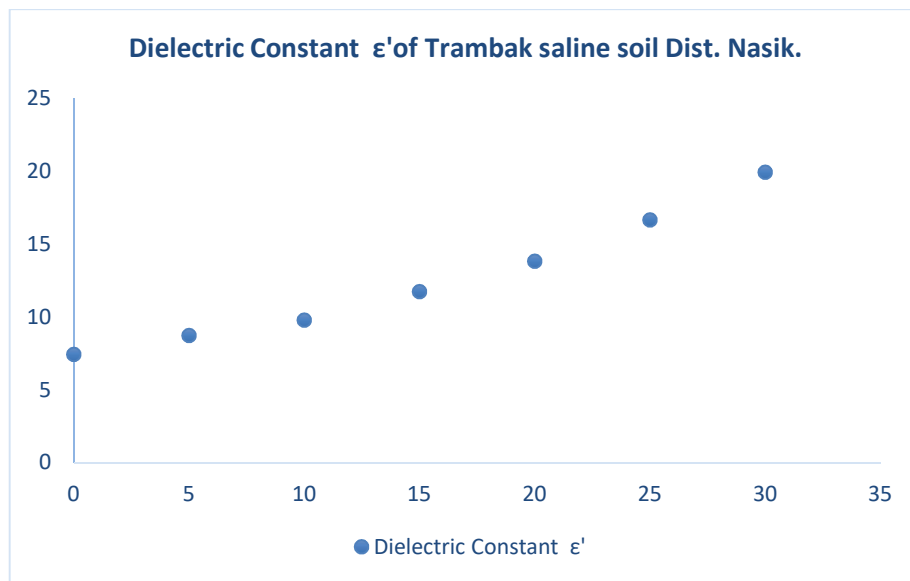
Figure 2 Variations of dielectric constant Versus Moisture% contain of Trambak District Nasik Saline soil saline soil.
