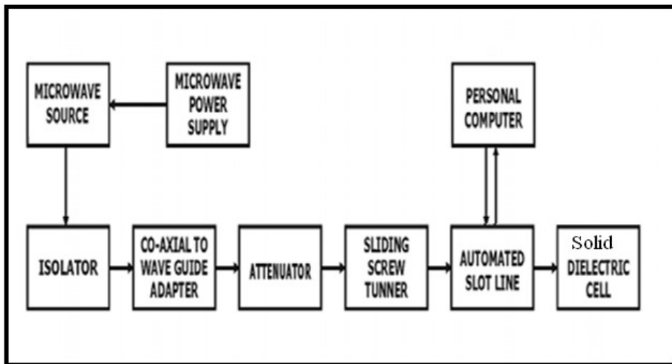
Figure 1 Block diagram of a C-band microwave bench
